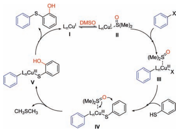
Scheme 2. Possible Mechanism
